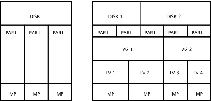
Figure 15.3 Physical Partitioning versus LVM
