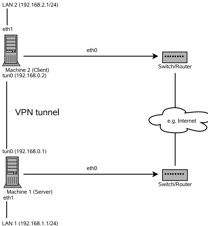
Figure 16.1 Routed VPN
