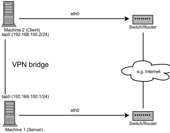
Figure 16.3 Bridged VPN - Scenario 2
