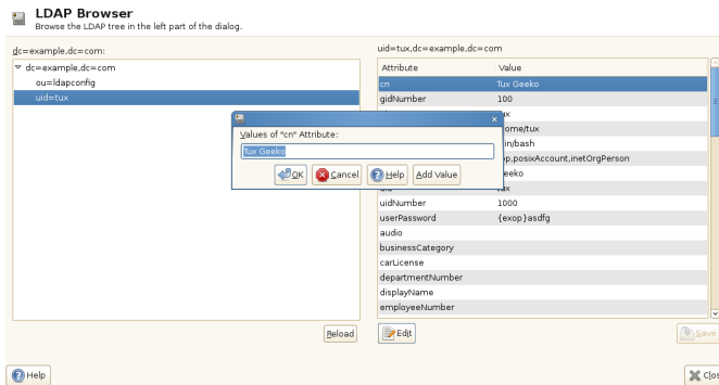
Figure 4.12 Browsing the Entry Data
