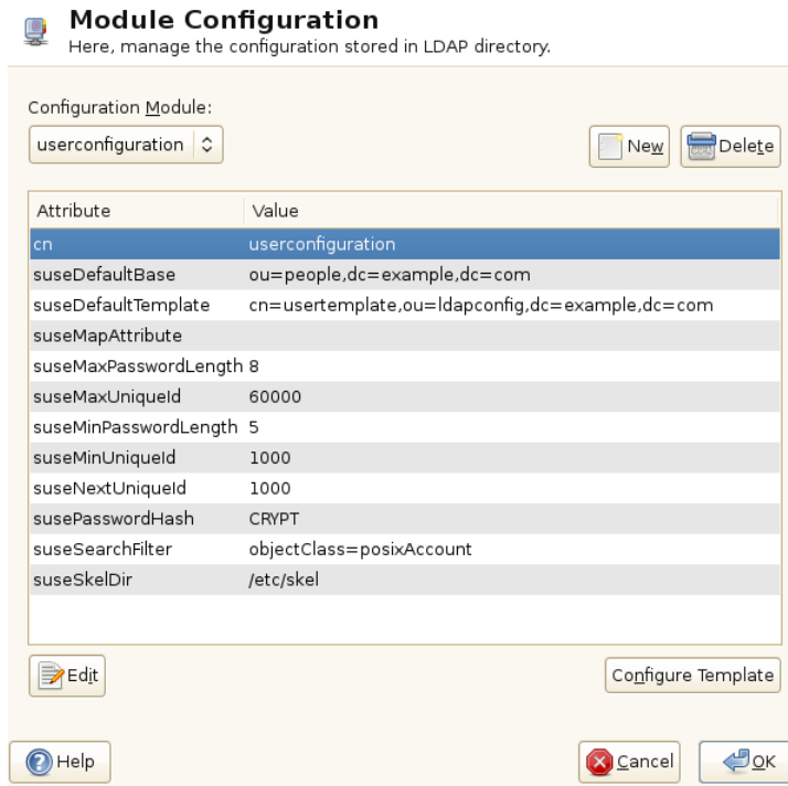
Figure 4.8 YaST: Module Configuration
