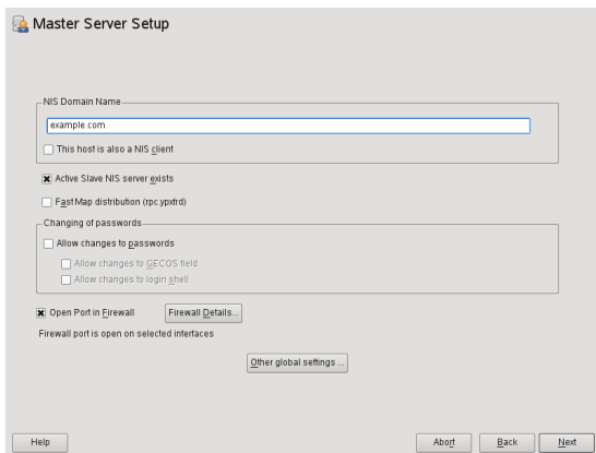
Figure 3.2 Master Server Setup
