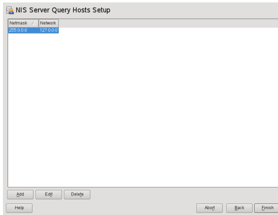
Figure 3.5 Setting Request Permissions for a NIS Server
