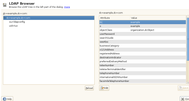
Figure 4.11 Browsing the LDAP Directory Tree
