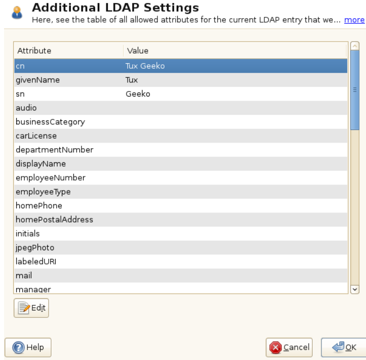
Figure 4.10 YaST: Additional LDAP Settings
