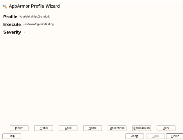
Figure 23.3 Learning Mode Exception: Defining Execute Permissions for an Entry
