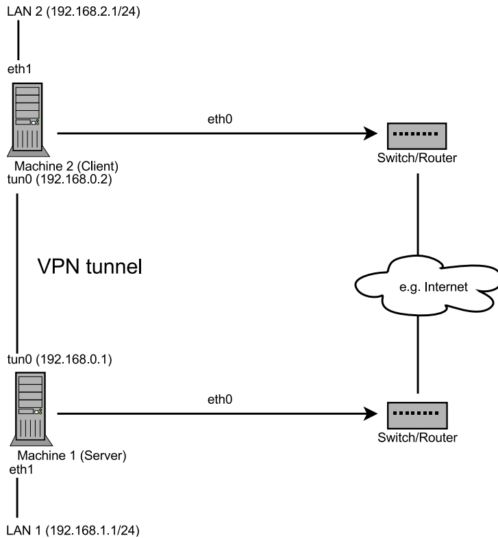
Figure 16.1 Routed VPN
