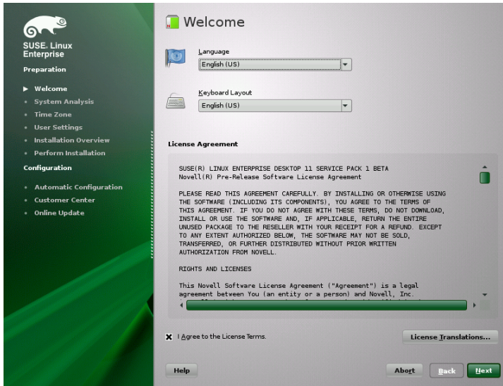
Figure 3.2 Welcome
