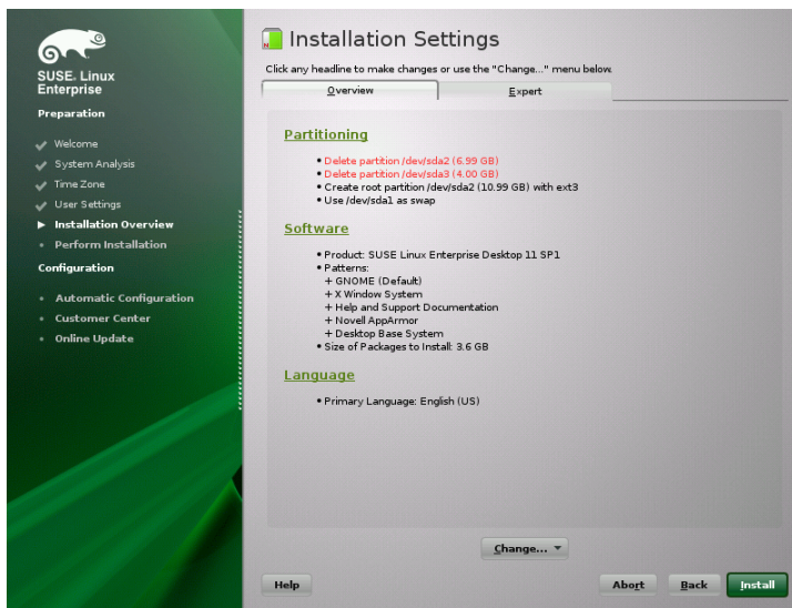
Figure 3.6 Installation Settings
