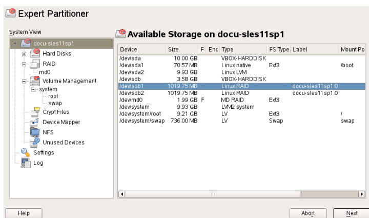
Figure 12.5 RAID Partitions
